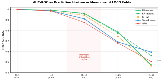
Fig. 8: AUC-ROC vs. prediction horizon for all models. All models converge near 1.0 at H=1 (trivially easy). H=10 (1 s) is the practical sweet spot: models diverge and the prediction remains actionable for wing actuation. At H=50 (5 s), all models approach random chance.
