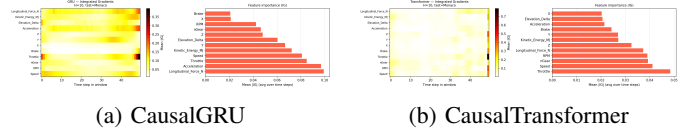
Fig. 7: Integrated Gradients attribution at Monaco ( H=10 ). (a) GRU ranks Longitudinal_Force and Acceleration highest — dynamic trajectory signals calibrated to fast training circuits. (b) Transformer ranks Throttle, Speed, and nGear highest — instantaneous state signals circuit-independent by design. This divergence explains the differential generalisation.
