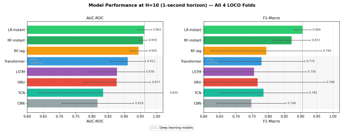
Fig. 5: Mean AUC-ROC at H=10 for all eight models with \pm 1\sigma error bars across LOCO circuits. LR-instant achieves the highest mean (0.963) and smallest standard deviation ( \pm 0.021 ). Deep learning models show larger variance.
