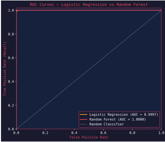
Fig. 4: ROC curves for Phase 1 current-mode classifiers. Both curves reach the top-left corner. Random Forest: AUC = 1.0000 (perfect); LR: AUC = 0.9997.
